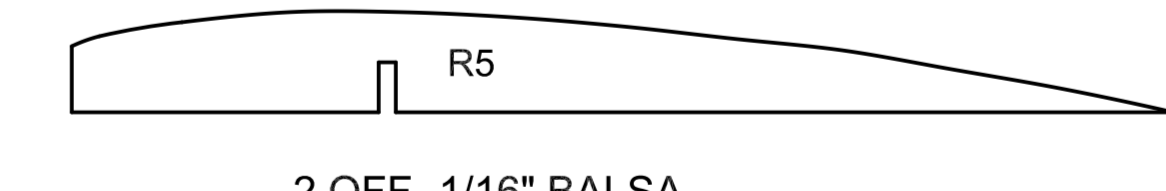
2 OFF - 1/16" Balsa
