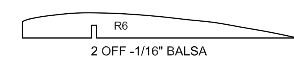
2 OFF - 1/16" Balsa
